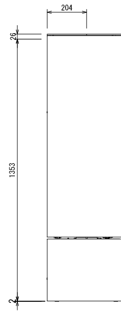
SIDE
